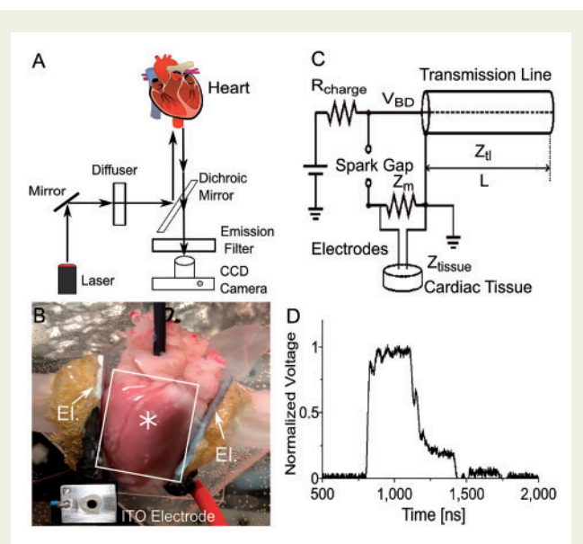
Figure 1 Setup used in our defibrillation experiments. (A) Optical mapping setup. The heart is stained with the voltage-sensitive fluorescent probe Di-4-ANBDQBS and illuminated with a diffused laser at 671 nm. Fluorescent light is filtered with a long pass filter and recorded with a CCD camera. (B) Photograph of heart in setup. The electrodes are positioned to the left and to the right of the heart (see arrows labelled 'El.'). illumination is from the top, and fluorescent light is also recorded from the top. Two aluminium plate electrodes touch the heart at the right and left ventricular free wall. Inset shows indium tin oxide (ITO) window electrode for observation of shock effects right under the electrode. A circular hole was drilled into the aluminium electrode and covered with glass that was coated with (electrically conductive) ITO. The label 'asterisks' indicates where the ITO electrode was located when it was used. The white rectangle indicates a typical field of view of the camera. (C) Spark gap generator for 300 ns shocks. (D) Experimentally determined shock waveform.
