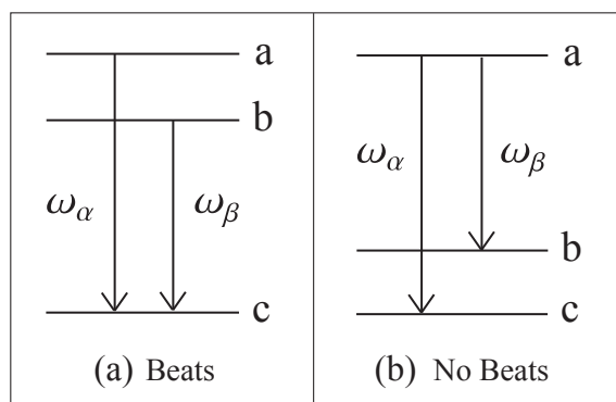
Fig. 5. Quantum beats – a) When a single atom decays from either of two upper levels to a common lower level, the two transition frequencies produce a beat note \omega_\alpha - \omega_\beta in the emitted photon. b) No beats are present when the lower levels are distinct, since the final state of the atom provides distinguishing information on the decay route taken by the photon.
