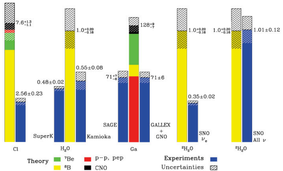
Total Rates: Standard Model vs. Experiment Bahcall-Pinsonneault 2000
