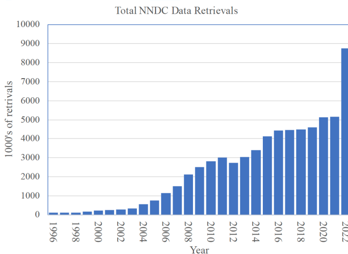
Figure 11.1. Total NNDC data retrievals per year from the USNDP databases at the NNDC from 1996 through 2022 [47].
