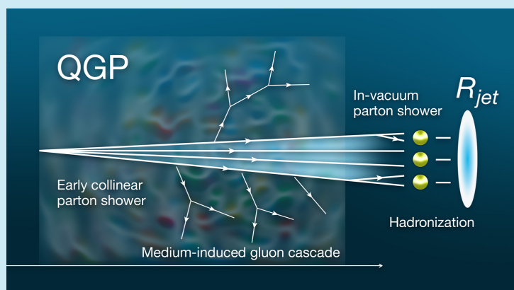
Figure 1. Schematic of jet evolution and interaction with quark–gluon plasma [S13].
