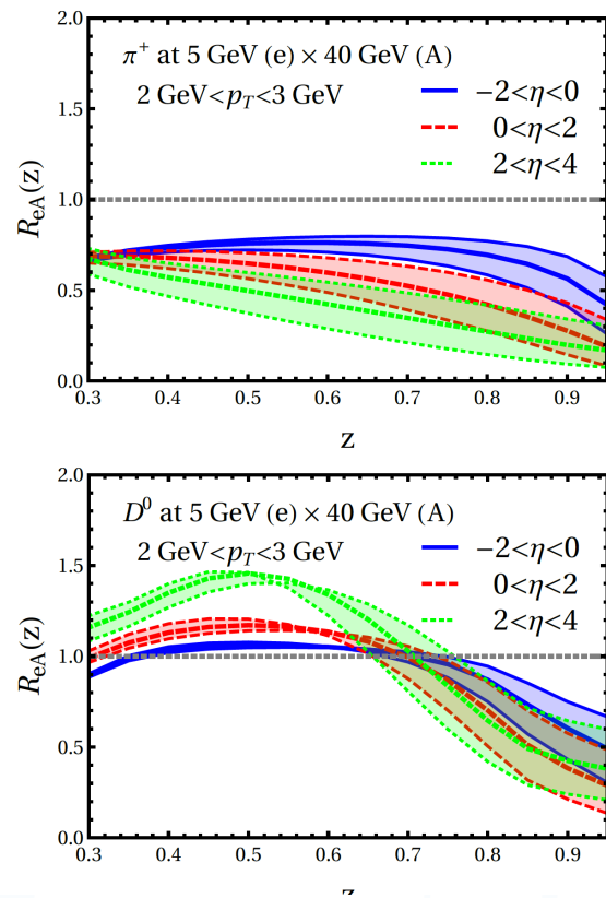
Figure 3.16. Predicted ratio of relative particle production ( N_h/N_{inc} ) in eA scattering over that in ep as a function of z , the momentum fraction of the parton carried by the respective hadron. Pions (top), which are light, show the largest nuclear suppression at the EIC. However, heavy flavor meson ratios (bottom) can differentiate models of hadronization since they show a substantially different modification in eA [16].
