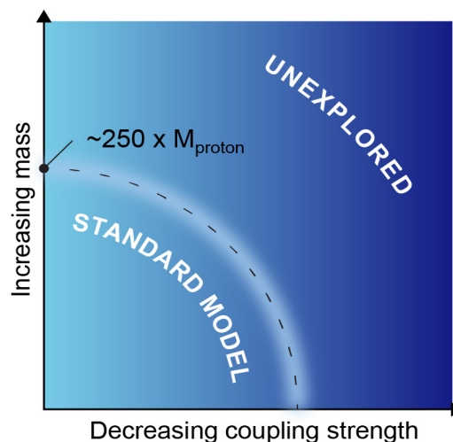
Figure 6.1. Physics beyond the Standard Model must reside at heavy masses and/or weak coupling strength. Physicists probe such regions through searches for rare and forbidden processes, high precision measurements of allowed processes, and exploration of properties of known and hypothetical particles [22].
